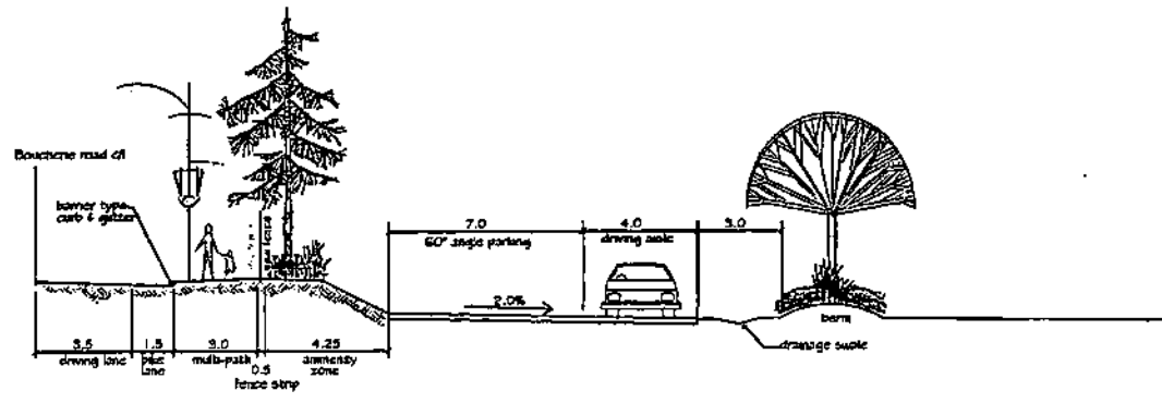
TYPICAL SITE SECTION
